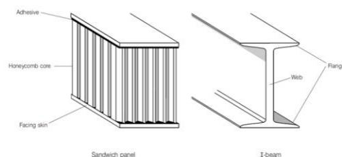
Figure 1.1 Sandwich Panel constructions
