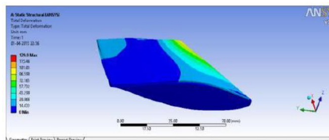
Figure 9.5 Deformation of the Of The Wing Box
