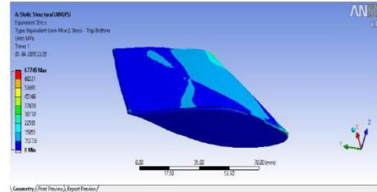
FIGURE 9.6 EQUIVALENT STRESS OF THE WING BOX
