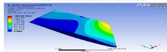
FIGURE 9.3 TOTAL DEFORMATION OF THE WING BOX
