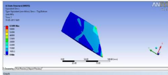
FIGURE 9.1 EQUIVALENT STRESS OF THE WING BOX
