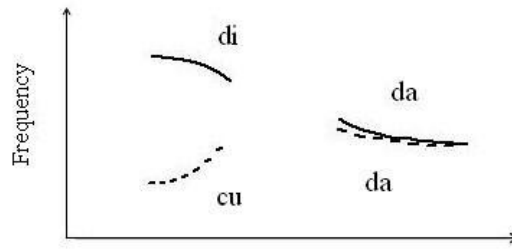
Fig. 2 F_2 contours of the sequence pair ‘dida’ and ‘cudā’, with the former in solid line, and the latter in dashed line
