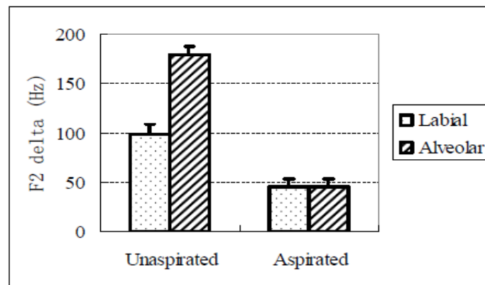
Fig. 6. F_2 delta under the effects of place of articulation and aspiration
